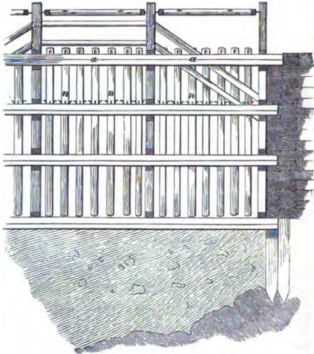
Fig. 259.—Boom with removable grating.
